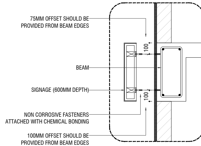
SIGNAGE DETAIL
